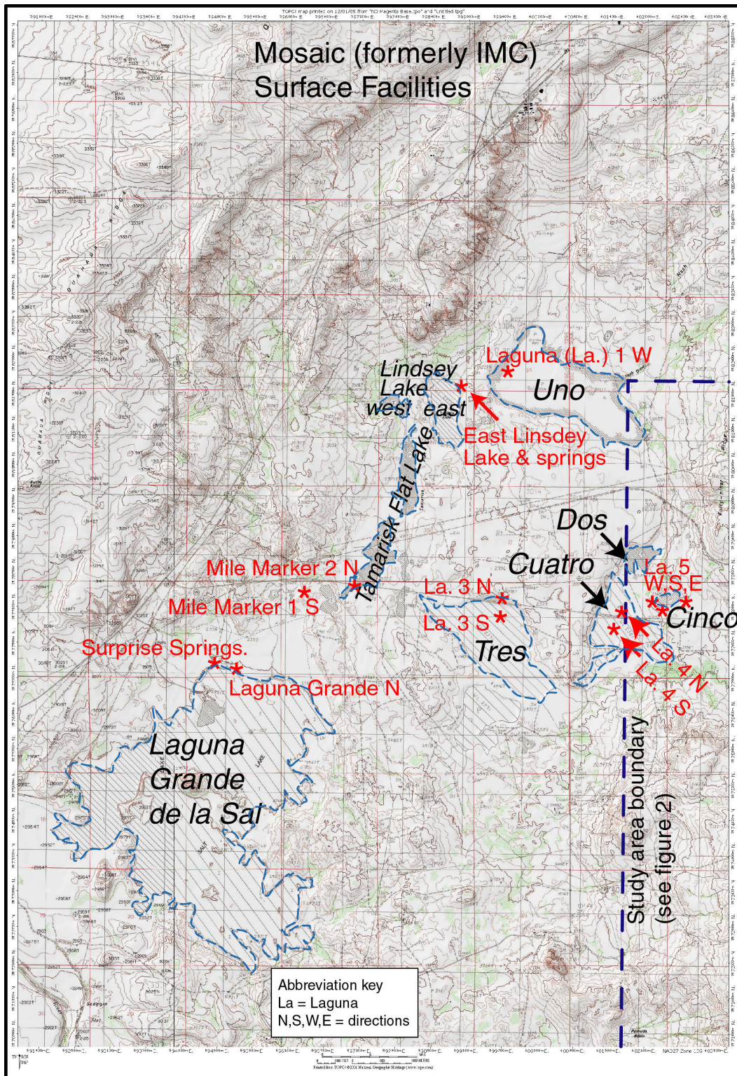
Figure 1. Brine ponds in southern Nash Draw. Red letters and asterisks identify general locations where historical specific gravity data have been collected since 1986. Major ponds are outlined with blue dashed lines.
