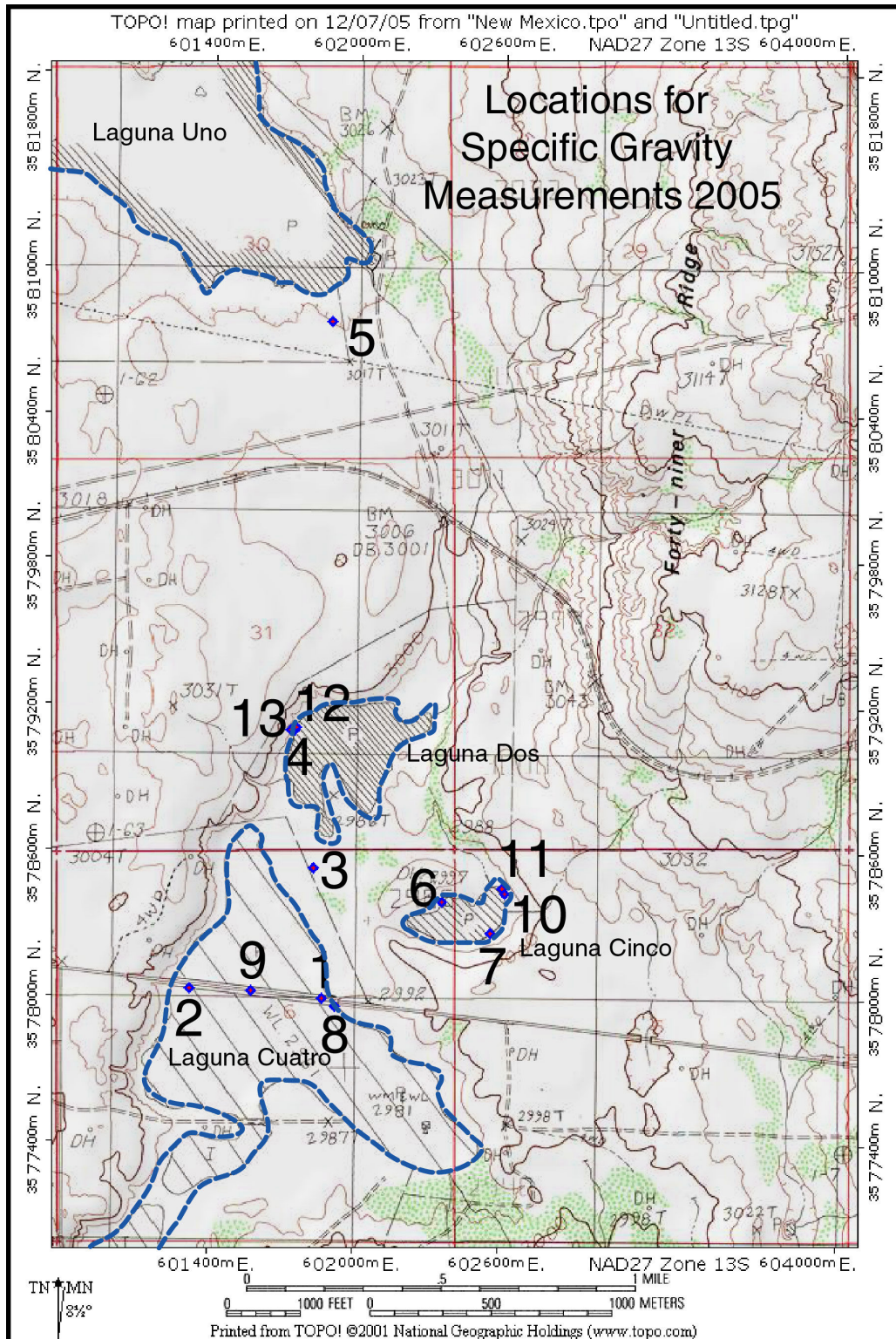
Figure 3 – Locations of specific gravity measurements. The locations are numbered according to the “sample #” listed in Tables 1 and 2. Locations 1-7 are approximately the same for both sample series listed in these tables.
