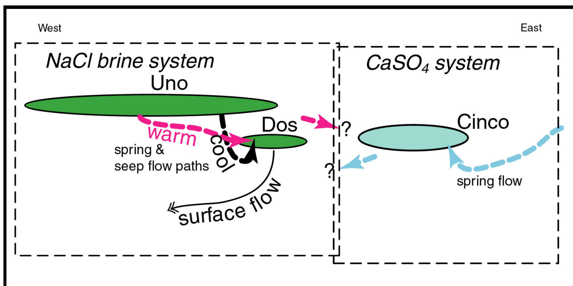
Figure 8. Diagrammatic concept of spring and seep flow. Laguna Uno, Dos, and other downgradient brine ponds are at or near saturation with respect to NaCl. Laguna Cinco has lower specific gravity and gypsum (sulfate) as a substrate. The NaCl system is maintained by potash tailings effluent into Laguna Uno. Laguna Cinco is recharged from karst in Rustler sulfate units. From Laguna Uno to Laguna Dos, there appear to be separate systems of cool flow that wells up in large springs in the bottom of Dos and warm seeps that travel in a shallower system.
