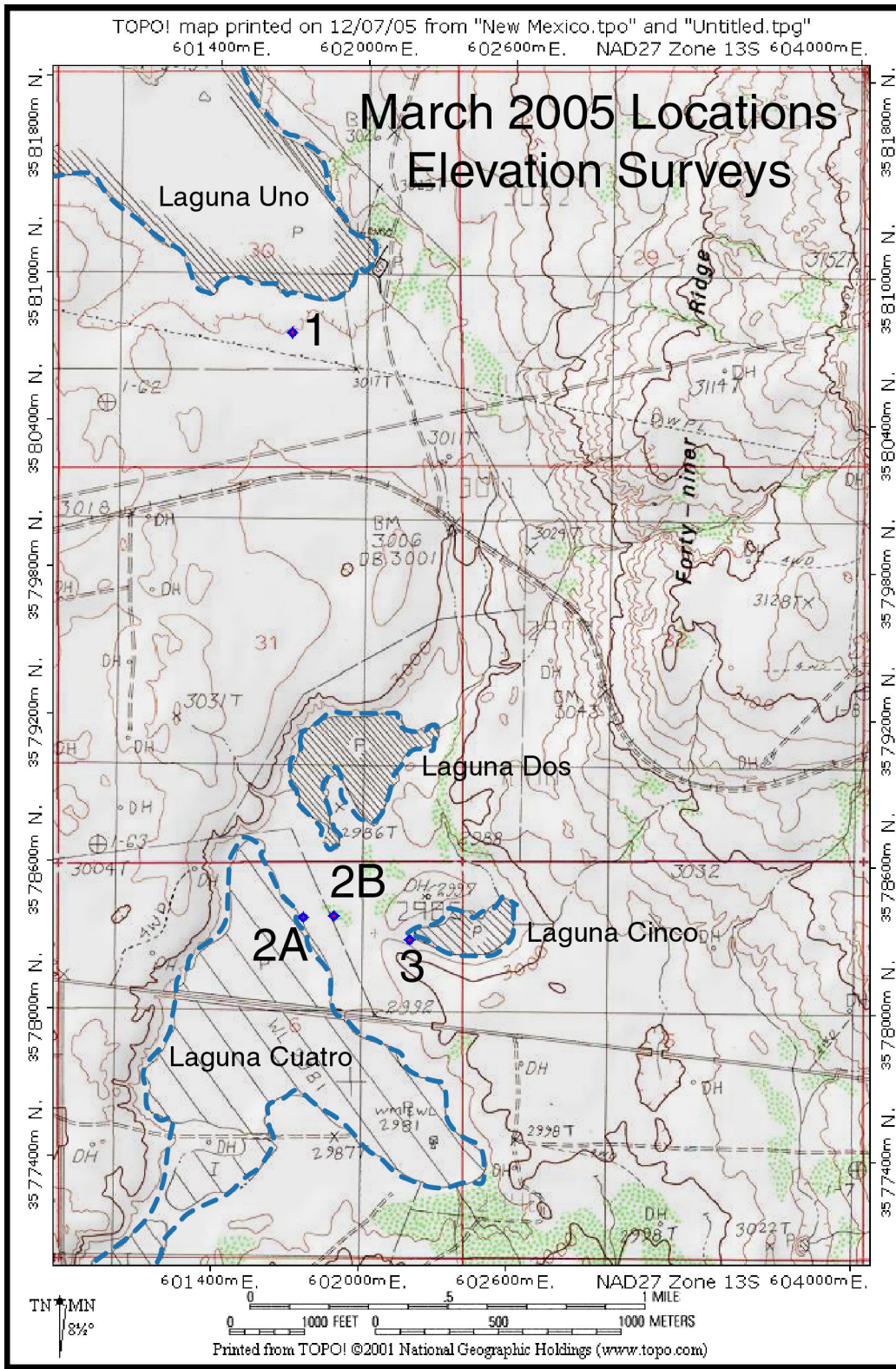
Figure 4 – Locations of brine lake elevation surveys. See Table 3 for location data and Figure 5 for a survey plat. Point 2B provides the elevation at the south end of Laguna Dos at higher water levels.
