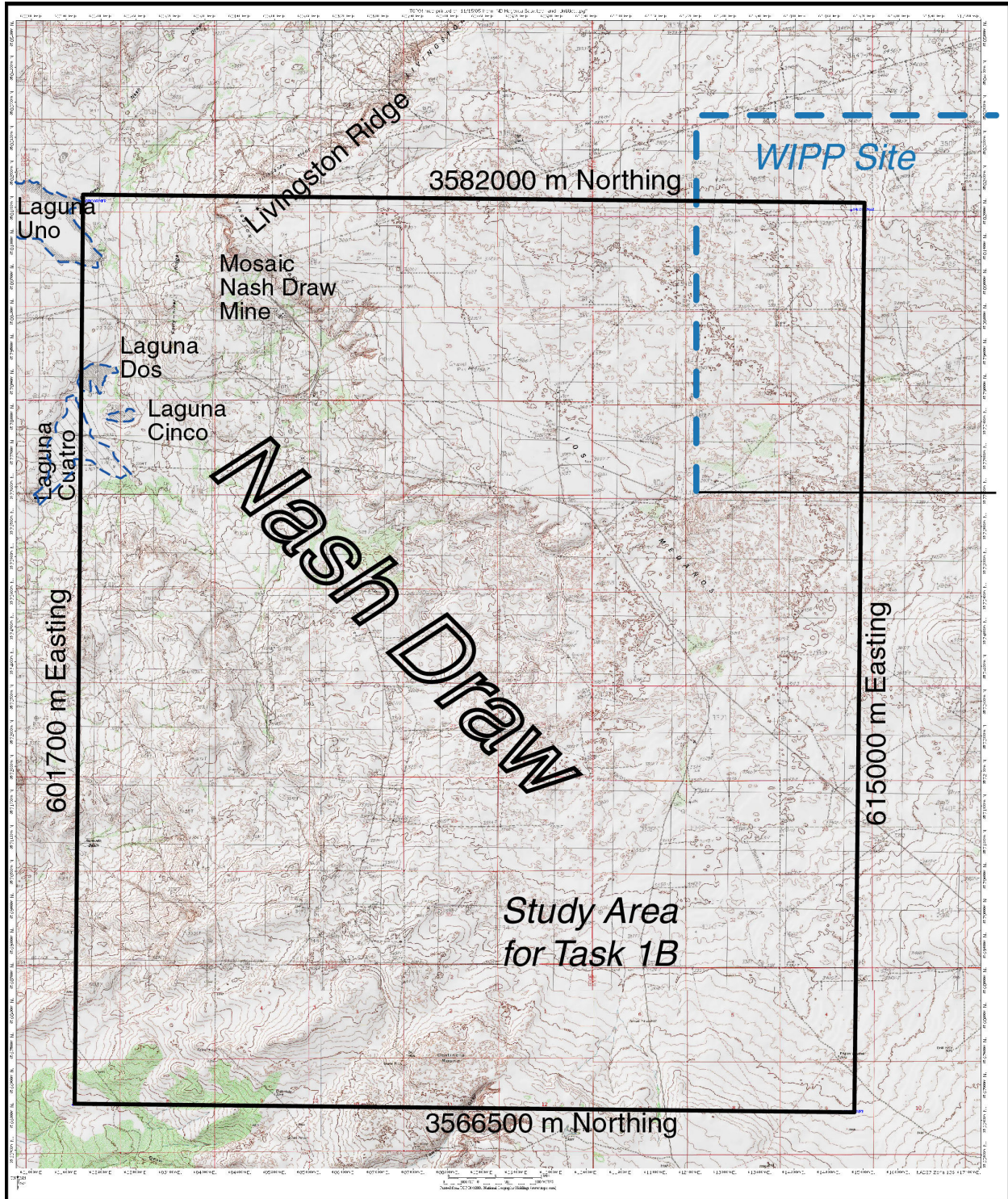
Figure 2 – Study area. The study area for Task 1B (Powers, 2006) shown in the black rectangle overlaps the southwestern part of the WIPP site (blue dashed outline) and is centered mainly on the southeastern arm of Nash Draw. Boundary limits are UTM (NAD27) coordinates in meters. Brine lakes described here as part of Task 1D occur in the northwestern corner of the study area.
