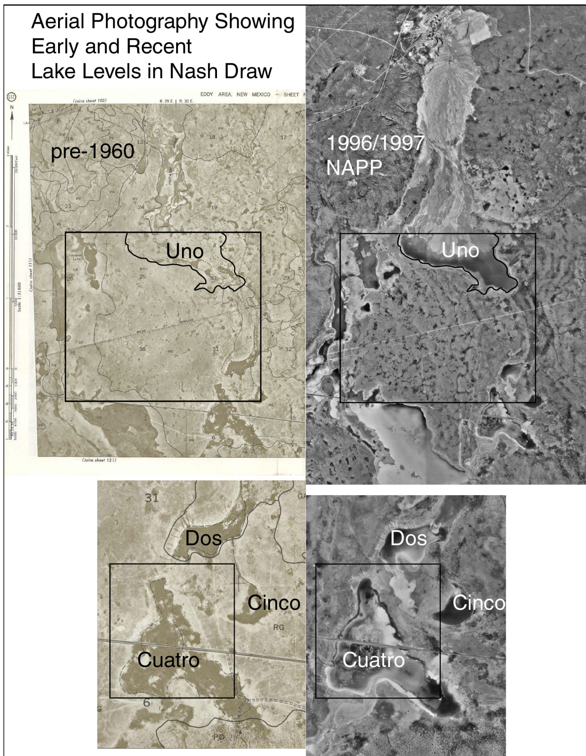
Figure 6 – Aerial photographs indicating historical changes in brine lakes. Squares show the corresponding points in photographs. The photos on the left are from Chugg et al. (1971; sheet 112) and pre-date 1960. The photos on the right are from the National Aerial Photograph Program (NAPP); this area is covered by photos 9615-12 (11/1/97) and 9611-51 (10/22/96).
