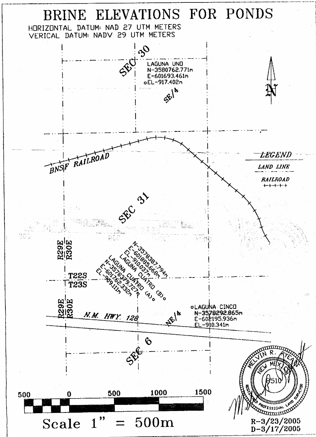
Figure 5 – Copy of survey plat by Melvin R. Pyeatt. The “Laguna Cuatro (B)” point is the southern edge of Laguna Dos, as it extends south to a slight rise that separates Laguna Dos from Laguna Cuatro. The survey was conducted March 2, 2005.
